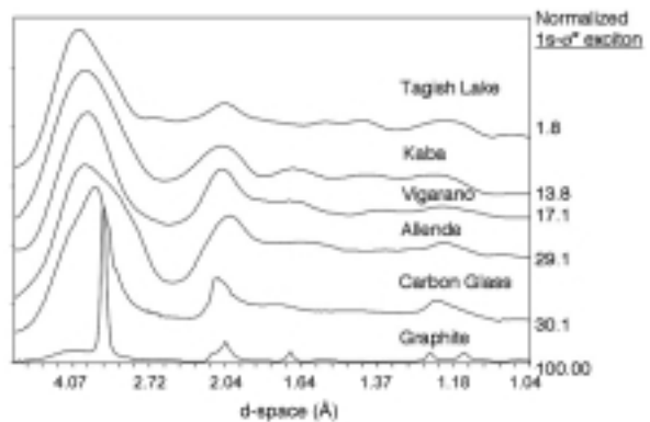
Fig. 9 X-ray diffraction data for a subset of IOM analyzed in this study (Cody et al. , 2008 b). Reproduced by permission from Elsevier.
