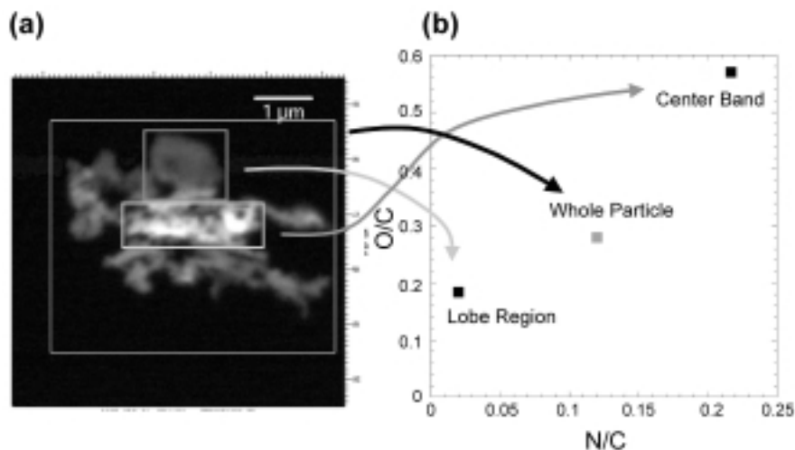
Fig. 4 a) An optical density image on the carbon (1 s) absorption edge of sample No. 5. b) Elemental data (N/C and O/C) from the “lobe region” and the “center band” (Cody et al. , 2008 a). Reproduced by permission from Meteoritics & Planetary Science, ©2008 by the Meteoritical Society.
