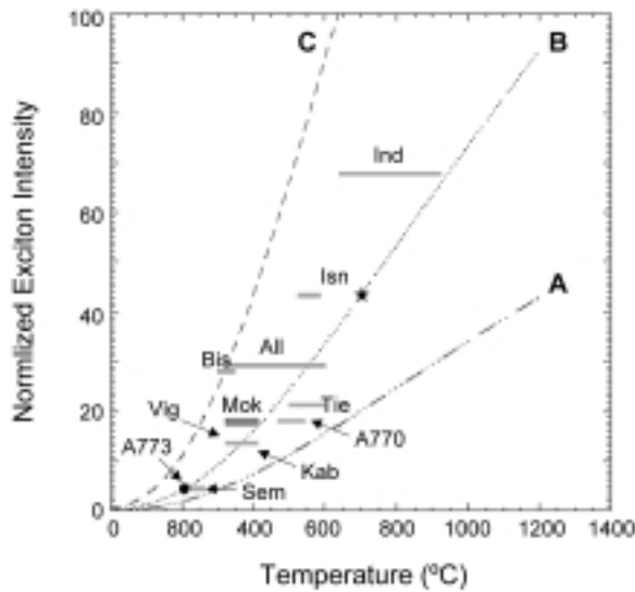
Fig. 7 The correlation between normalized exciton intensity (%) and various estimates of temperature (gray bars). Included is a single estimate for a temperature of Isna (black star) employing Fe/Mg partitioning between olivine-spinel grains. The petrologic type 1 and 2 chondrites in this study all fall into the gray region at the origin of the plot. Curves A, B, and C plot the predicted relationship between exciton intensity and temperature derived from the thermo-kinetic experiments. Curve A uses as determined kinetic parameters. Curves B and C are calibrated assuming that Isna's T_{\text{EFF}} = 700^\circ\text{C} and Allende's T_{\text{EFF}} = 325^\circ\text{C} , respectively (Cody et al. , 2008 b). Reproduced by permission from Elsevier.
