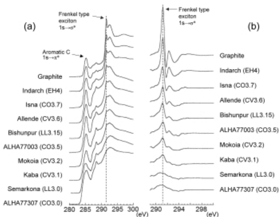
Fig. 6 (a) C-XANES spectra of type 3+ chondrites spanning the CO, CV, Ordinary, and enstatite chondrite groups. A reference spectrum of graphite is included on top. (b) The first derivative of the C-XANES spectra (from 289 to 300 eV) (Cody et al. , 2008 a). Reproduced by permission from Elsevier.
