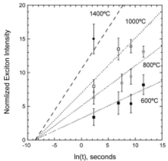
Fig. 8 The experimentally observed Log-linear time-temperature development of the 1s \rightarrow \sigma^* exciton in insoluble organic matter from IOM upon heating to 600 (■), 800 (■), and 1000 (□) ^\circ\text{C} for various times (Cody et al. , 2008 b). Reproduced by permission from Elsevier.
