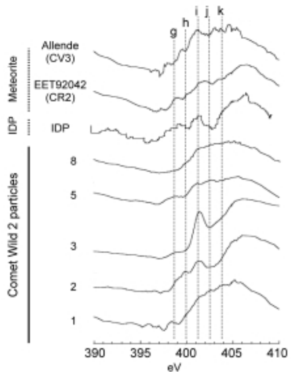
Fig. 2 N-XANES spectra obtained of organics associated with 81P/Wild 2 particles. Included for comparison are a spectrum of an anhydrous IDP (L2011 R11), and insoluble organic matter isolated from meteorites, CR2 (EET 92042) and CV3 (Allende). Peaks corresponding to specific functional groups are highlighted with the letters g - k. g: 1s-\pi^* transition at \sim 399 eV for imine, h: 1s-\pi^* transition at \sim 400 eV for nitrile, i: 1s-\pi^* transition at \sim 401.4 eV for amidyl nitrogen, j: 1s-\sigma^*/3p transition at \sim 402.5 eV for amino nitrogen, k: 1s-\sigma^*/3p transition at \sim 403.5 eV for urea (Cody et al. , 2008 a). Reproduced by permission from Meteoritics & Planetary Science, ©2008 by the Meteoritical Society.
