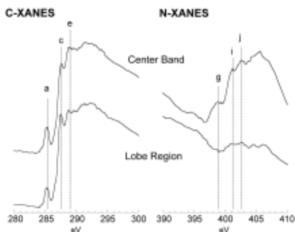
Fig. 5 a) C-XANES spectra of sample No. 5 “lobe” (bottom) and “center band” (top). b) N-XANES spectra of sample No. 5 “lobe” (bottom) and “center band” (top) (Cody et al. , 2008 a). Reproduced by permission from Meteoritics & Planetary Science, ©2008 by the Meteoritical Society.
