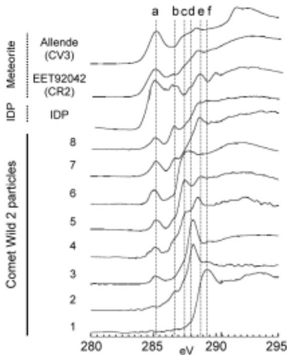
Fig. 1 C-XANES spectra of organics associated with Comet 81P/Wild 2 particles. Included for comparison are spectra of an anhydrous IDP (L2011 R11) and insoluble organic matter isolated from CR2 (EET 92042) and CV3 (Allende) chondrites. Peaks corresponding to specific functional groups are indicated with letters a-f. a: 1s-\pi^* transition at \sim 285 eV for aromatic carbon, b: 1s-\pi^* transition at \sim 286.7 eV for nitrile, c: 1s-3p/s^* at \sim 287.5 eV for aliphatic carbon, d: 1s-\pi^* transition at \sim 288.2 eV for carbonyl carbon in amide moieties, e: 1s-\pi^* transition at \sim 288.5 eV for carbonyl carbon in carboxyl or ester moieties, f: 1s-3p/s^* transition at \sim 289.5 eV for alcohol or ether moieties (Cody et al. , 2008 a). Reproduced by permission from Meteoritics & Planetary Science, ©2008 by the Meteoritical Society.
