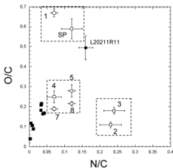
Fig. 3 Atomic N/C versus O/C derived from C-, N-, and O-XANES of organics associated with 81P/Wild 2 particles ( \square ). Included are elemental data for meteoritic organic matter isolated from types 1, 2, and 3 chondrites ( \blacksquare ) and the anhydrous IDP L2011 R11 ( \blacklozenge ) (Cody et al. , 2008 a). Reproduced by permission from Meteoritics & Planetary Science, ©2008 by the Meteoritical Society.
