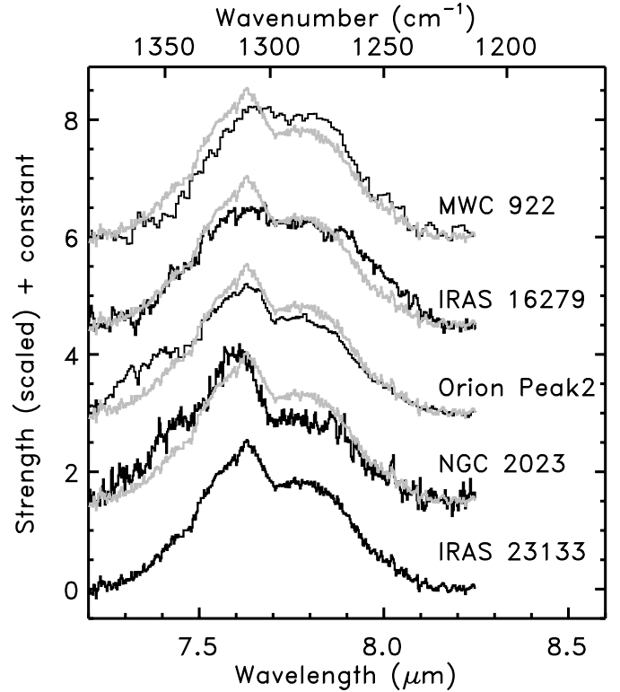
Fig. 13. The typical – normalised – profile of the 7.7 \mu\text{m} complex of class A' represented by IRAS 23133, shown together with the particular cases within this class. As a reference, the typical A' profile of IRAS 23133 is plotted on top of each profile in grey.
