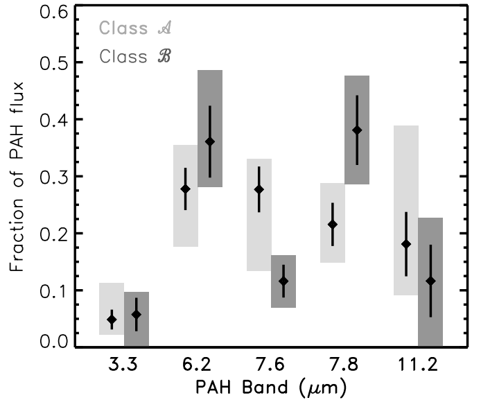
Fig. 19. An overview of the fraction of the PAH flux emitted in each feature for class \mathcal{A} and class \mathcal{B} . The diamonds crossed by solid vertical lines represent the average fraction of the total PAH flux emitted in each PAH band over a given class and its standard deviation. The filled boxes represent the observed ranges of the fraction of PAH flux emitted in each PAH band within a class. Light grey represents class \mathcal{A} and dark grey class \mathcal{B} . For the total PAH flux, we considered the 3.3, 6.2, 7.7 and 11.2 \mu\text{m} features.
