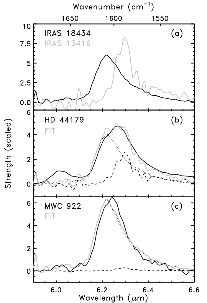
Fig. 10. Panel a ) shows the two components used for fitting the normalised profiles in class B. Panels b ) and c ) show the normalised profiles of HD 44179 and MWC 922 respectively together with the fit and the two components, reflecting their respective contributions. The spectra are interpolated to the same wavelength grid of resolution 500.
