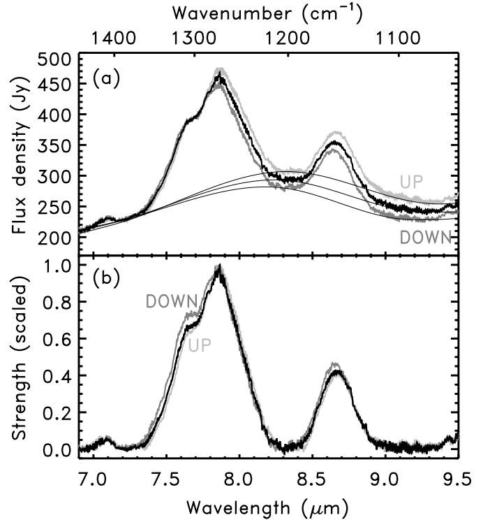
Fig. 2. The combined spectrum of HD 44179 (black line) together with the – independently reduced – up and down scans are shown with their respective continua in panel a). The continuum subtracted profiles are shown in panel b) normalised to the peak intensity.
